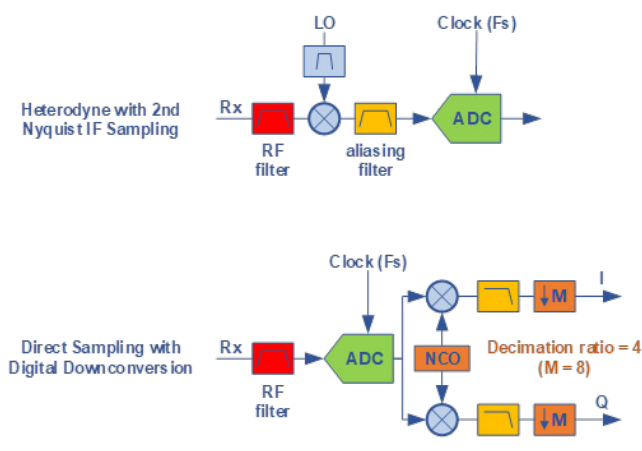
Figure 1 - Simplified Rx signal chains in a) traditional single stage heterodyne radio with mixer down conversion and b) a direct conversion system exploiting sampled signal aliasing within the ADC.
