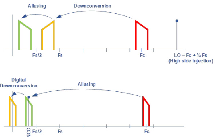
Figure 1 - Simplified Rx signal chains in a) traditional single stage heterodyne radio with mixer down conversion and b) a direct conversion system exploiting sampled signal aliasing within the ADC.
