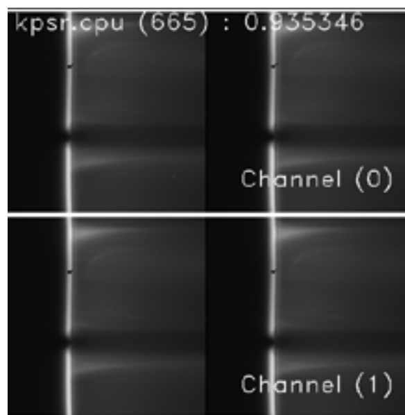
Figure 3 : Example of coronal mass ejection detection.
