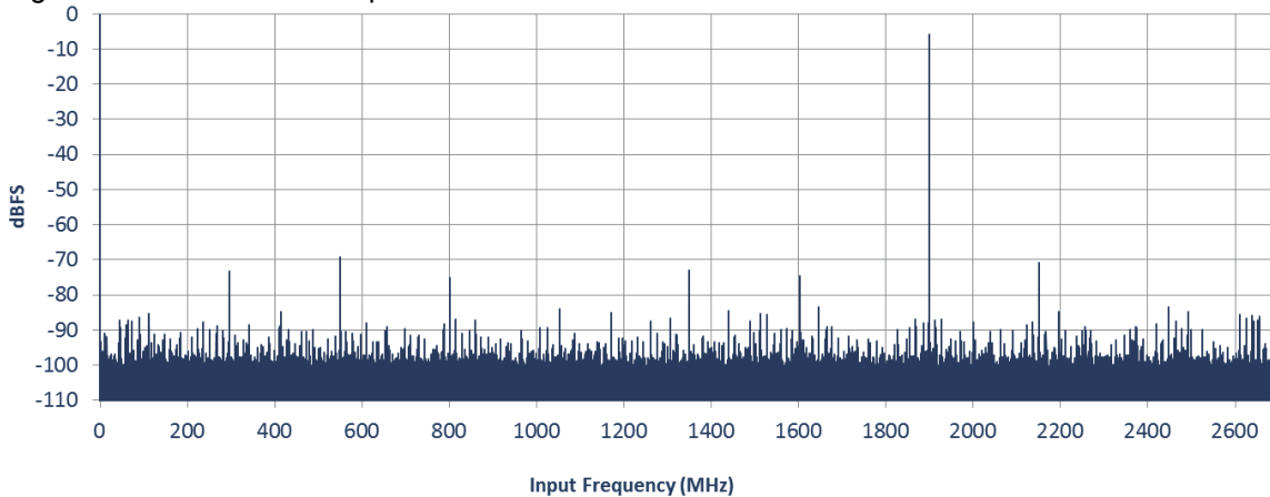
Figure 37. FFT at 5.4GSps and F_{in} = 1900\text{MHz} / -6\text{dBFS}
