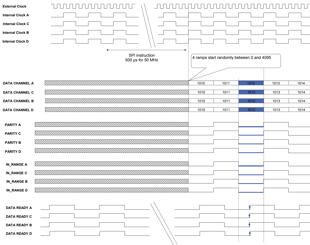
Figure 13. ADC Timing in ramp mode with 4 ADC cores sampling the same signal
