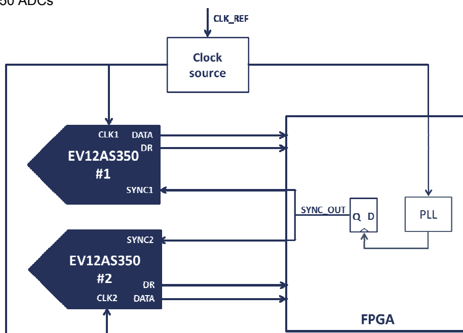
Figure 59. Example of multi-ADC synchronization using synchronous SYNC signals with 2 synchronous EV12AS350 ADCs
