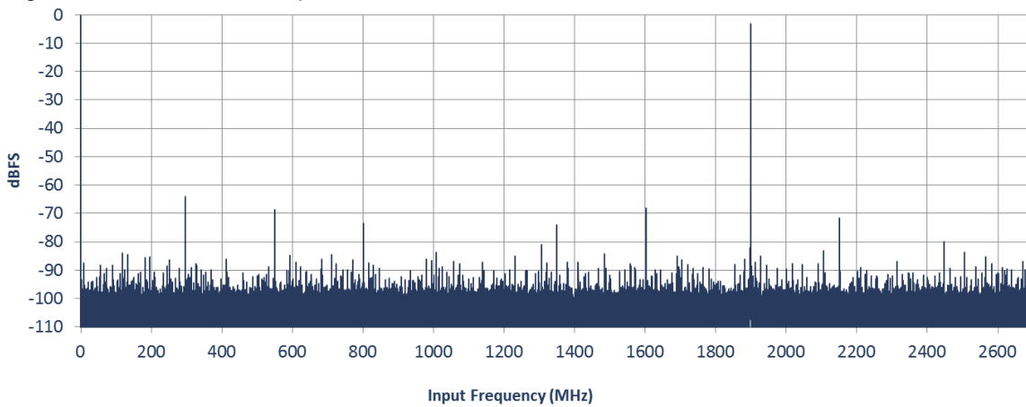
Figure 36. FFT at 5.4GSps and F_{in} = 1900\text{MHz} / -3\text{dBFS}
