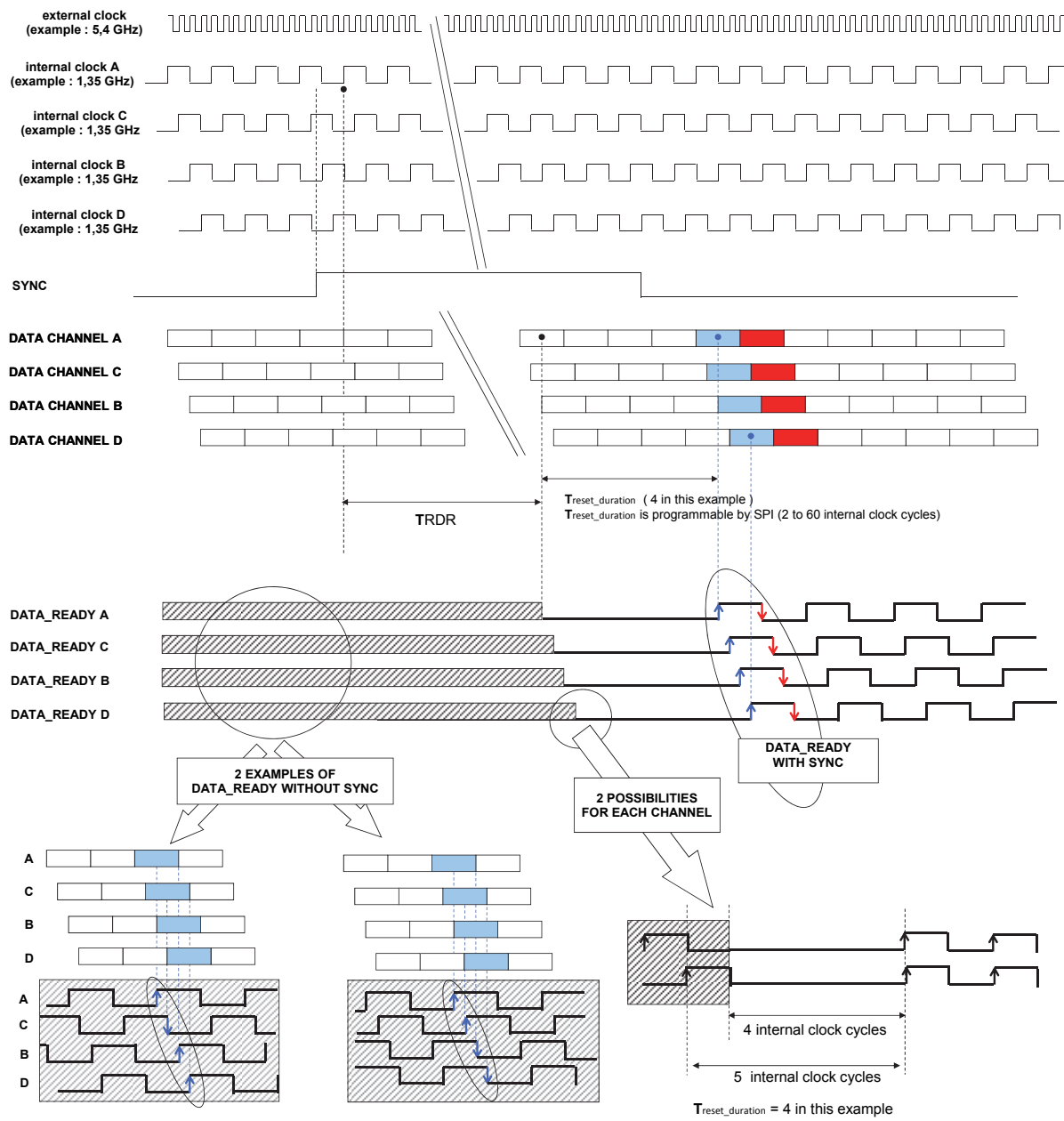
Figure 11. ADC Timing in flash mode with 4 ADC cores sampling the same signal
