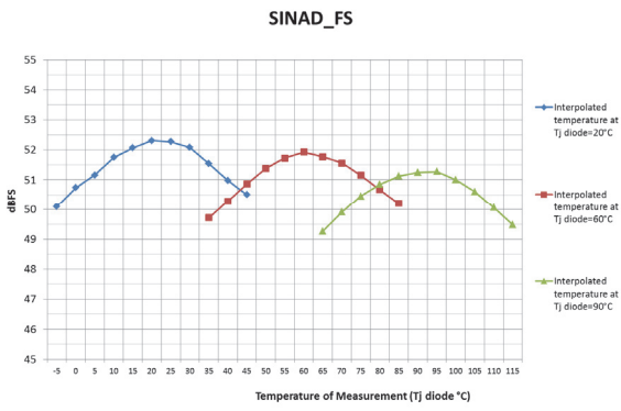
Versus Temperature - Typical supplies - 4 cores interleaved (Staggered mode).
