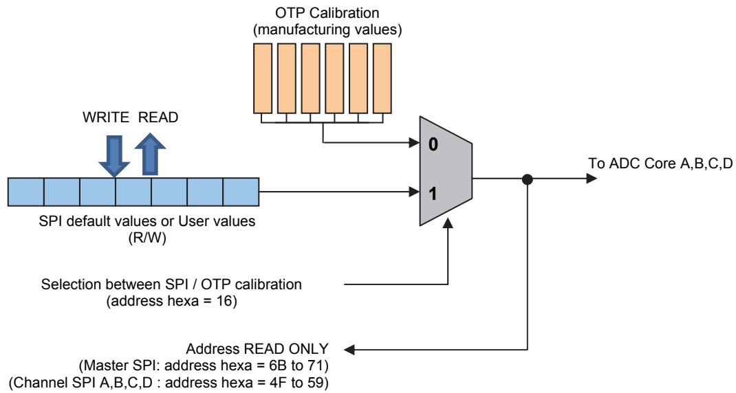
Figure 17. Selection between OTP and SPI registers
