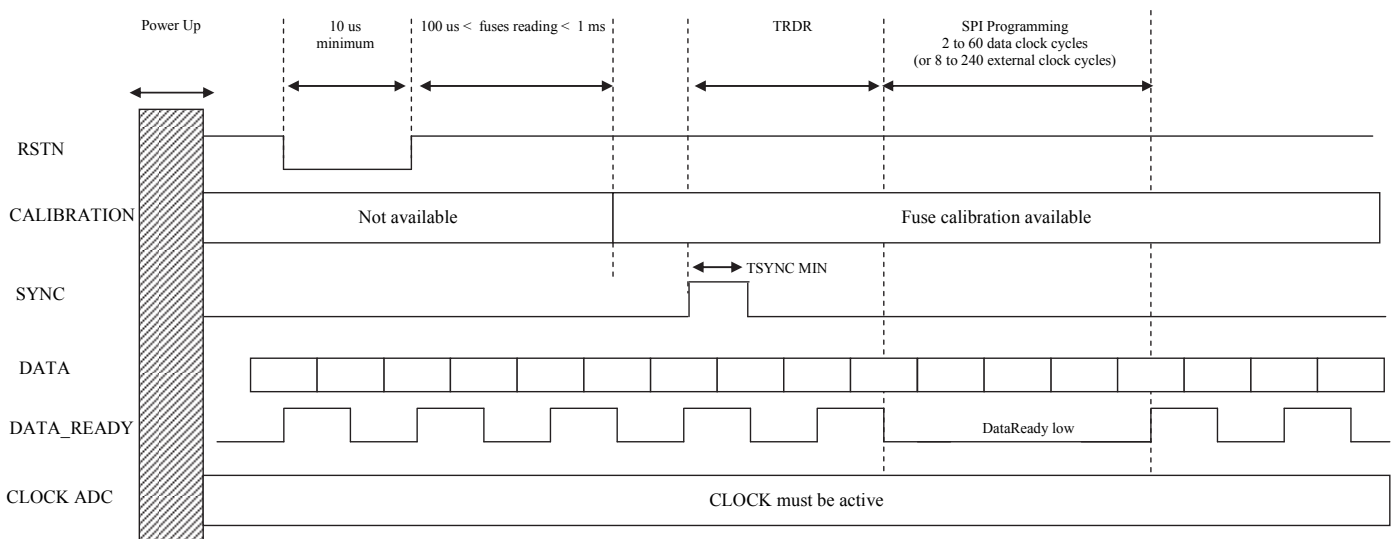
Figure 19. Software reset and start up procedure
