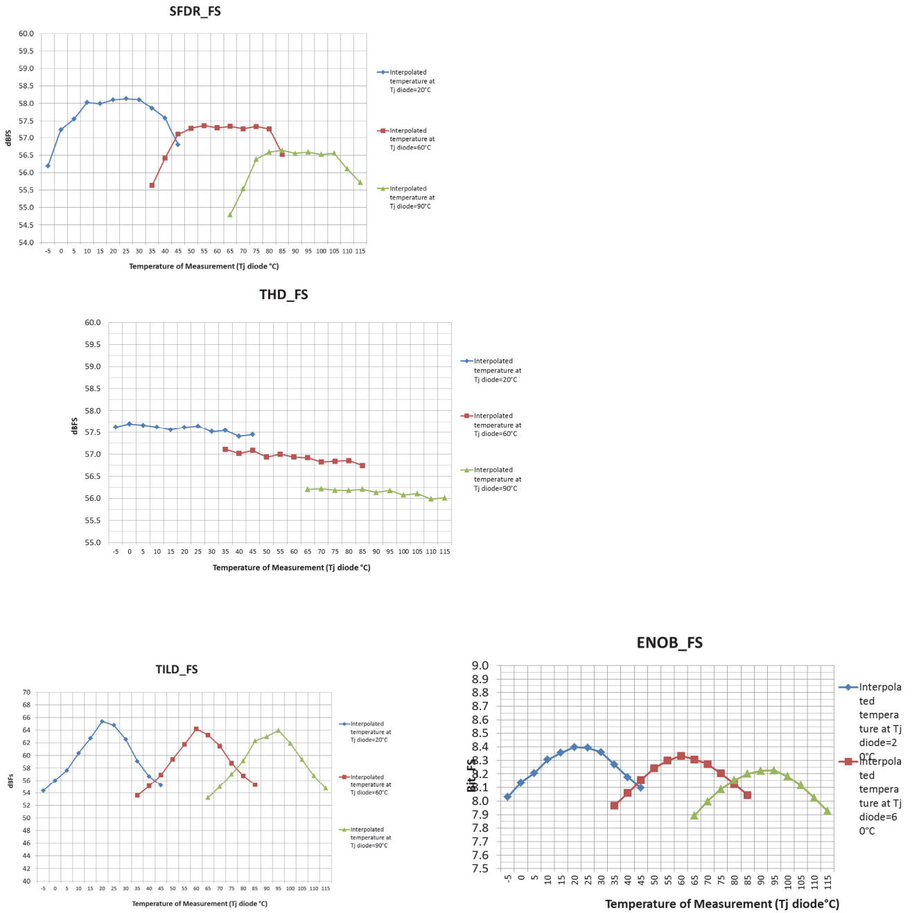
Figure 44. Impact of the temperature interpolation on SFDR, THD, TILD, ENOB, SINAD and SNR performances. F_c = 5\text{Gps} , F_{in} = 1900\text{MHz} , A_{in} = -1\text{dBFS}
