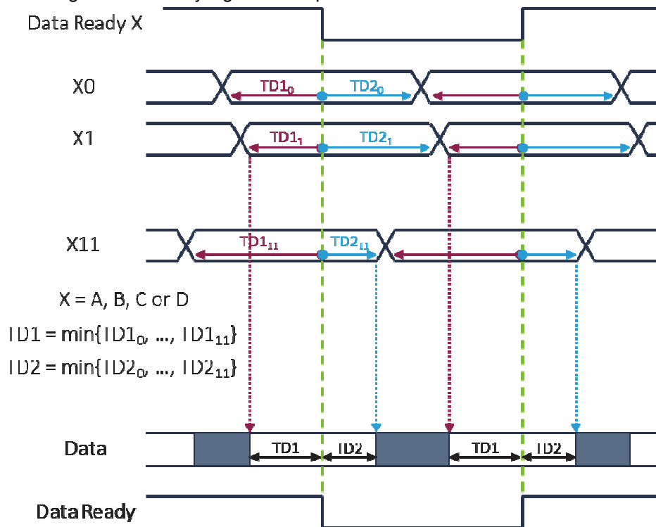
Figure 7. Centering of Data Ready signal on output data
