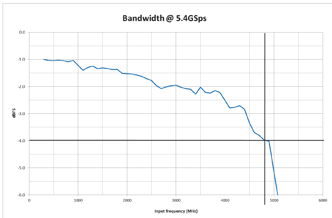
Figure 30. Bandwidth up to 4800MHz
