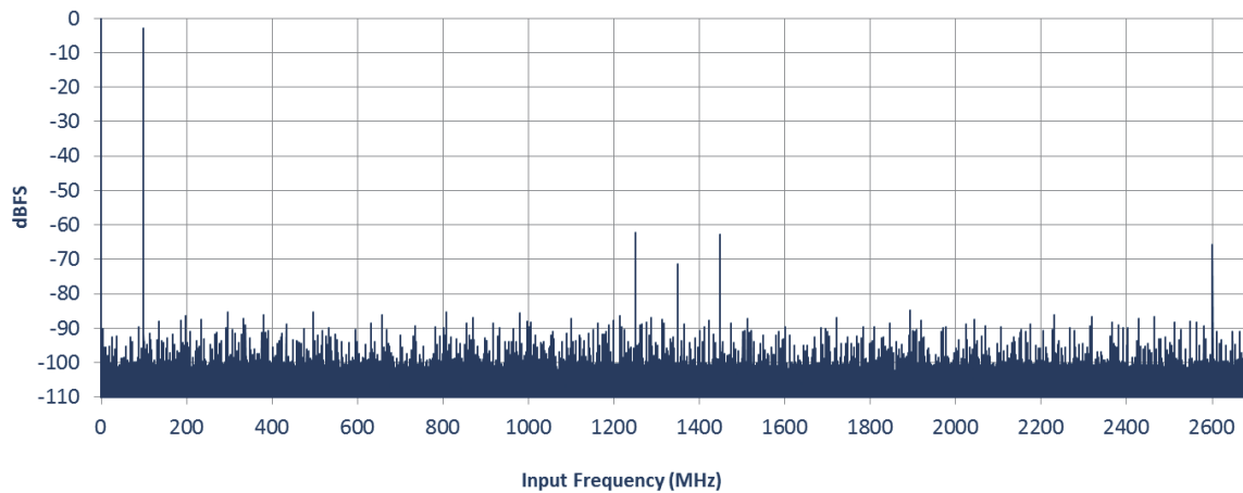
Figure 33. FFT at 5.4GSps and F_{in} = 100\text{MHz} / -3\text{dBFS}
