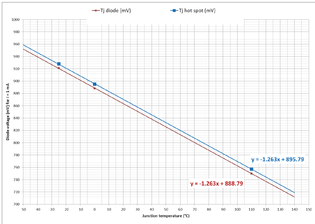
Figure 28. Temperature diode characteristics for I=1 mA (with DiodeC=GND)
