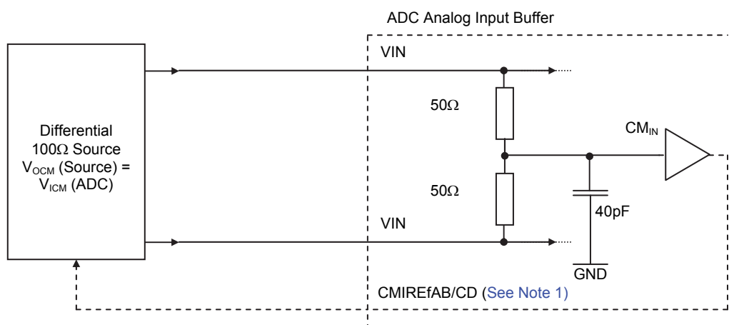
Figure 55. Differential analog input implementation (DC coupled)
