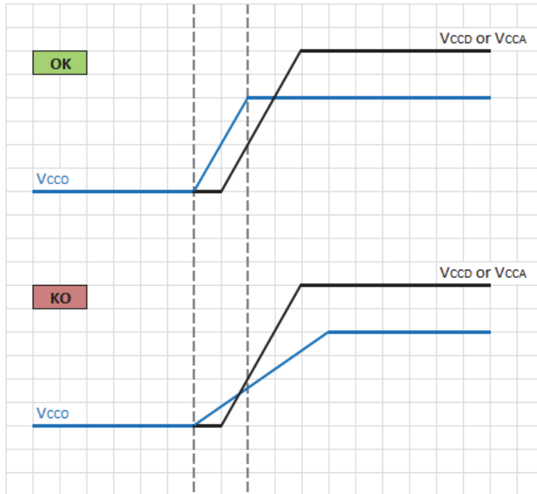
Figure 53. EV12AS350 Power-up sequencing
