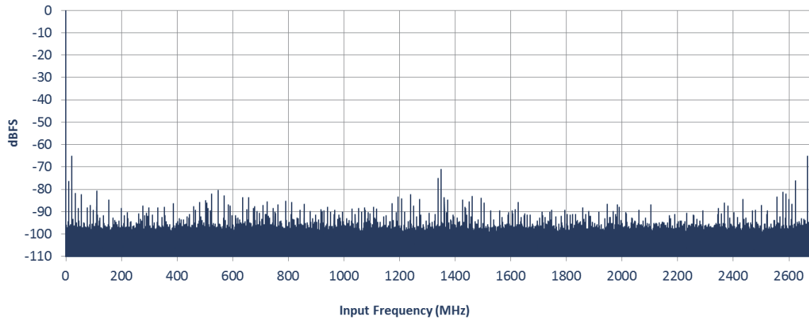
Figure 40. FFT at 5.4GSps and F_{in} = 2690\text{MHz} / -6\text{dBFS}
