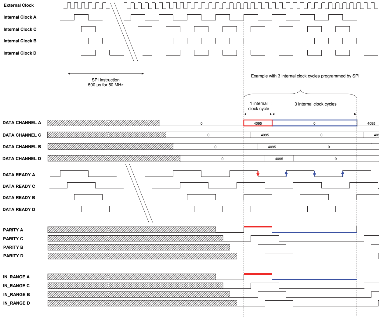
Figure 10. ADC Timing in Flash mode with 4 ADC cores interleaved
