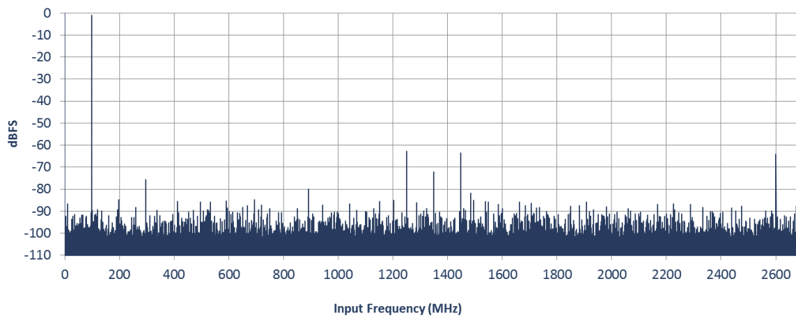
Figure 32. FFT at 5.4GSps and F_{in} = 100\text{MHz} / -1\text{dBFS}
