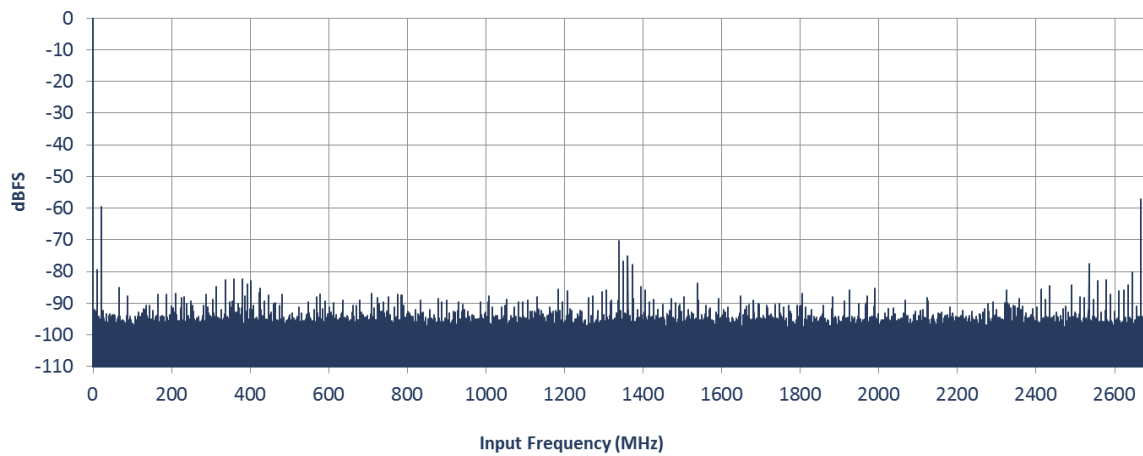
Figure 39. FFT at 5.4GSps and F_{in} = 2690\text{MHz} / -3\text{dBFS}
