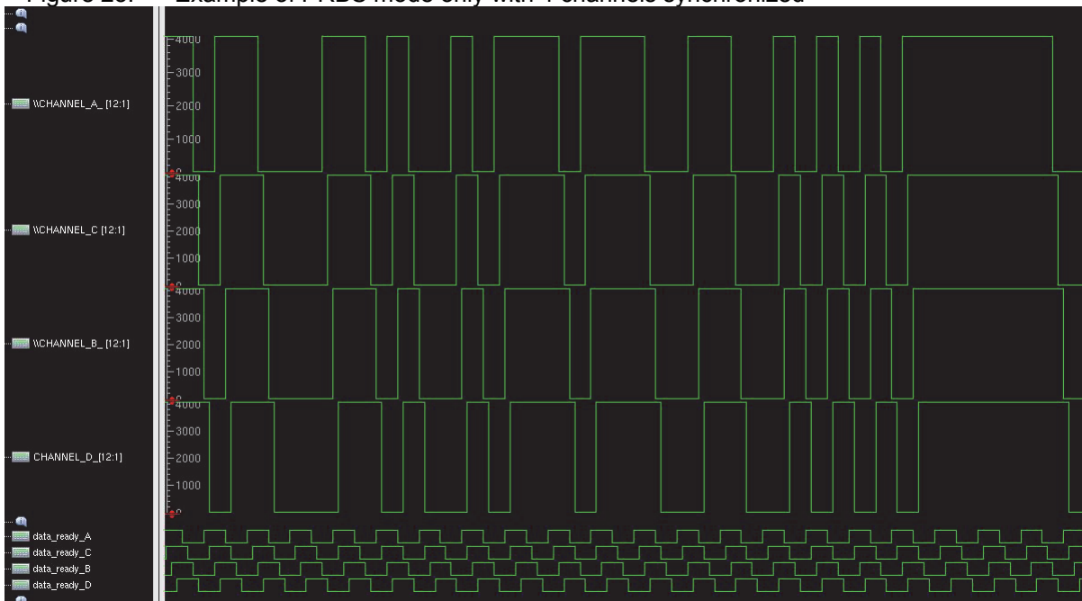
Figure 25. Example of PRBS mode only with 4 channels synchronized
