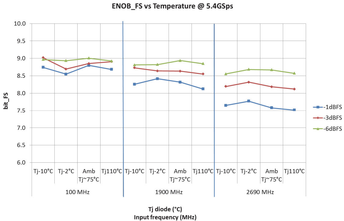
Figure 43. ENOB performance versus temperature These acquisitions are done at typical supplies in 4 cores interleaved (Staggered mode).
