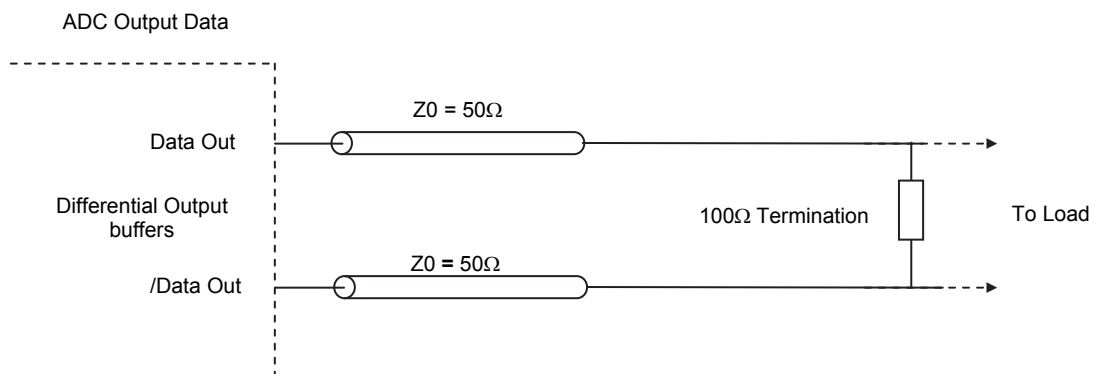
Figure 57. Differential digital outputs Terminations (100Ω LVDS)
