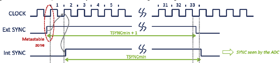
Figure 20. Example of an asynchronous SYNC signal rising in a metastable zone
