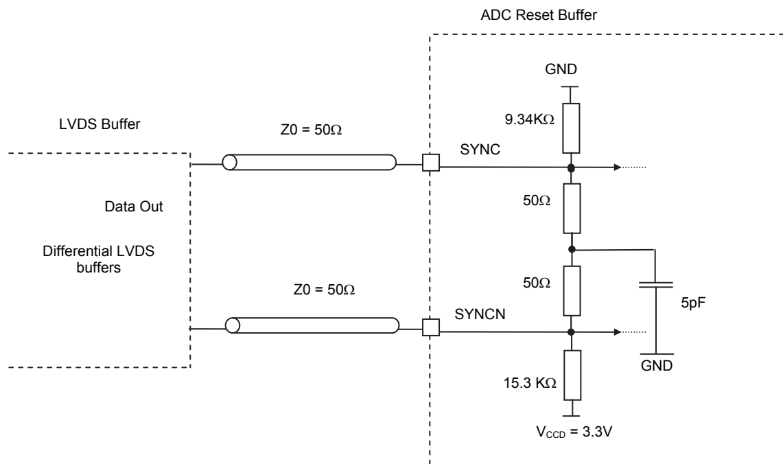
Figure 58. Reset Buffer (SYNC, SYNCN)
