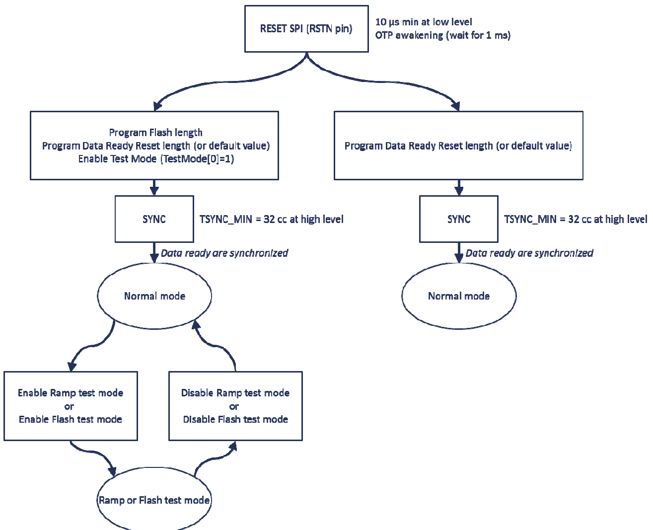
Figure 18. Software reset and start up procedure diagram
