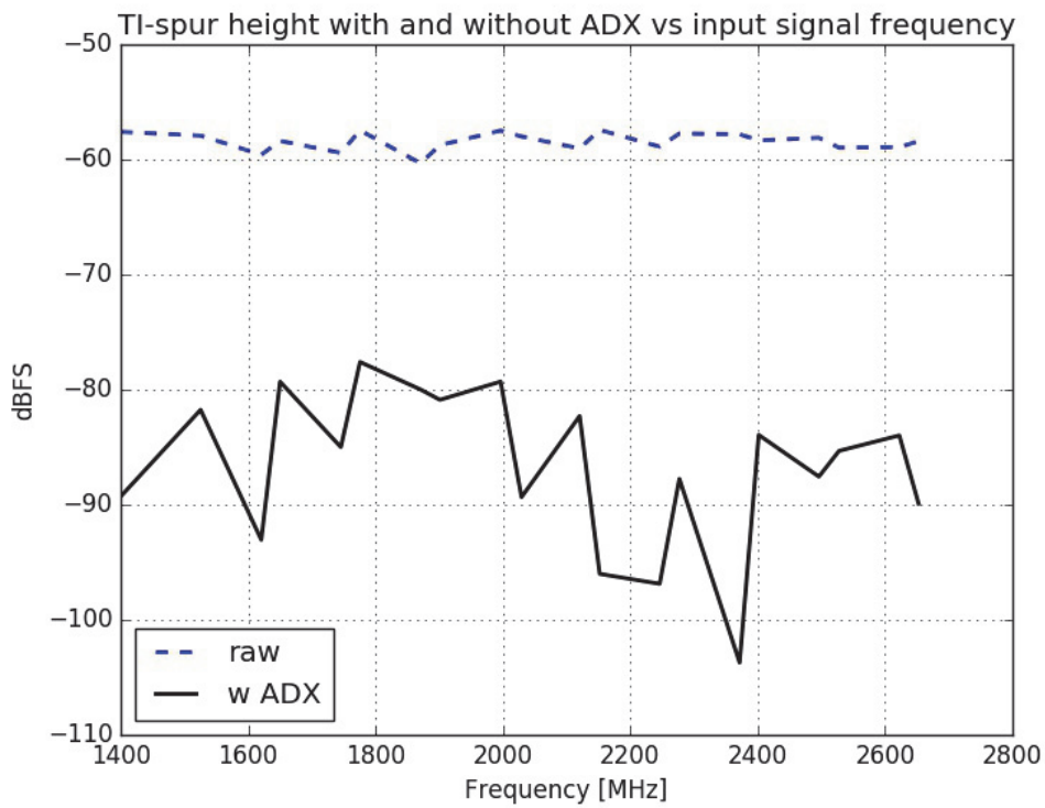
Figure 50. TI-spur height with and without ADX4 vs input signal frequency at 5.4Gps
