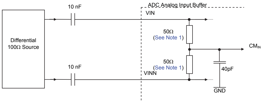
Figure 54. Differential analog input implementation (AC coupled)
