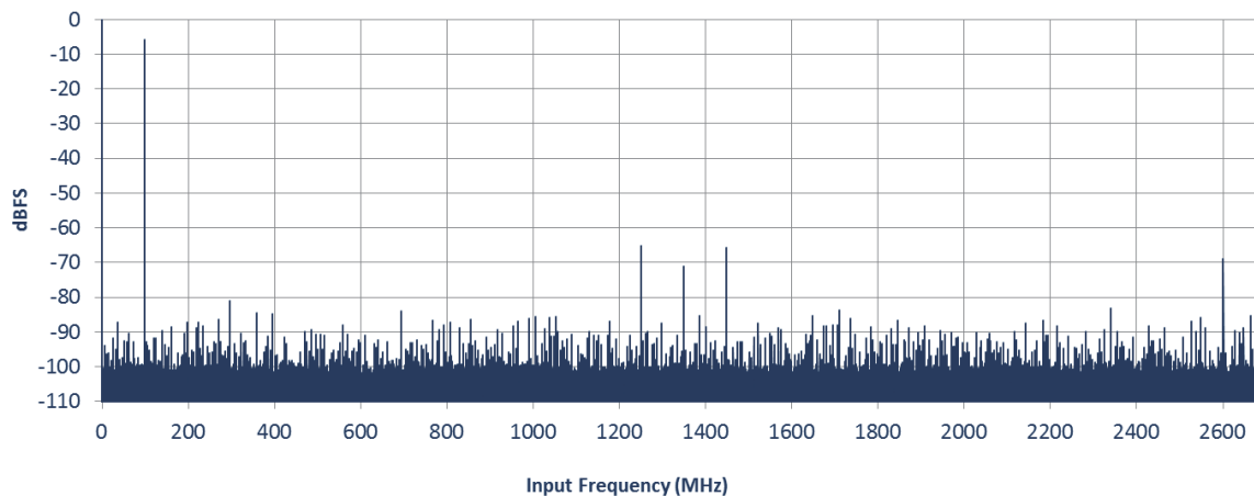
Figure 34. FFT at 5.4GSps and F_{in} = 100\text{MHz} / -6\text{dBFS}
