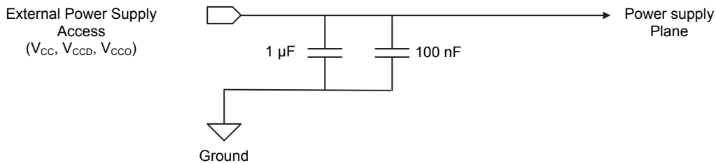
Figure 51. EV12AS350 Power supplies Decoupling and grounding Scheme
