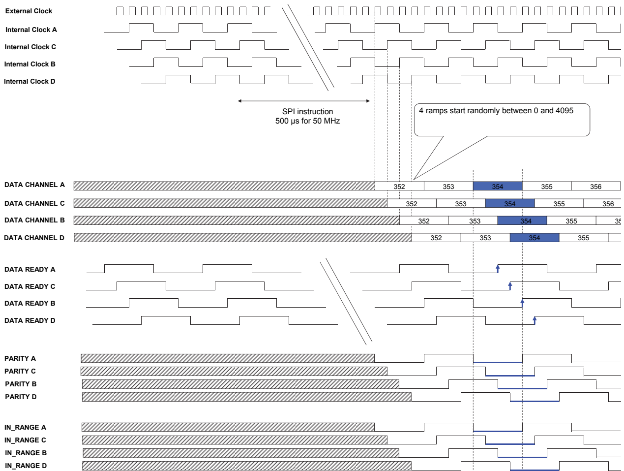
Figure 12. ADC Timing in ramp mode with 4 ADC cores interleaved
