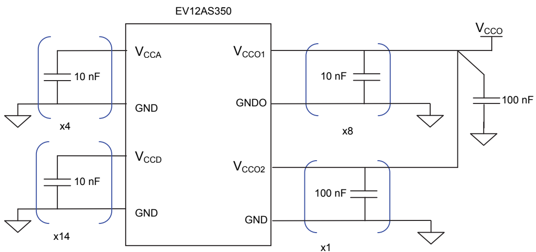
Figure 52. EV12AS350 Power Supplies Bypassing recommended Scheme
