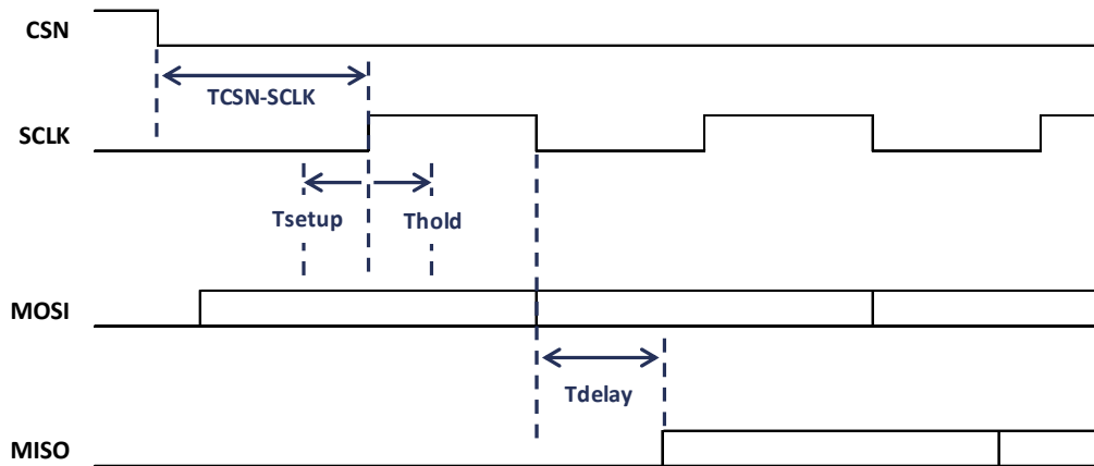
Figure 4. SPI Timing Diagram
