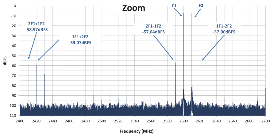
Typical supplies - at ambient temperature - 4 cores interleaved (Staggered mode).
