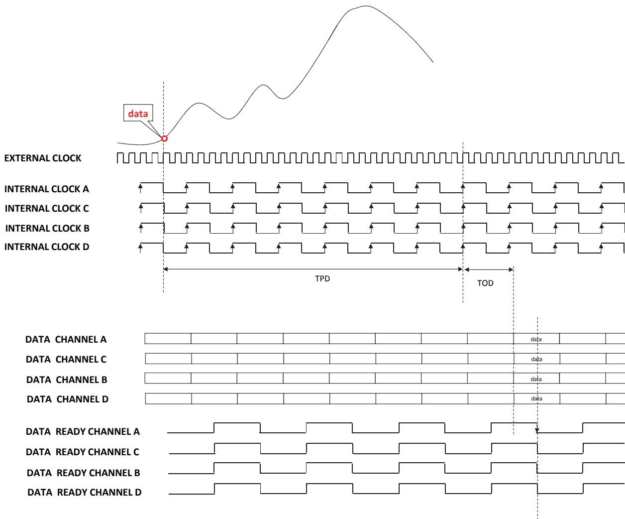
Figure 6. ADC Timing in simultaneous mode or simultaneous sampling (4 ADC cores sampling the same signal)
