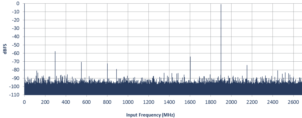
Figure 35. FFT at 5.4GSps and F_{in} = 1900\text{MHz} / -1\text{dBFS}
