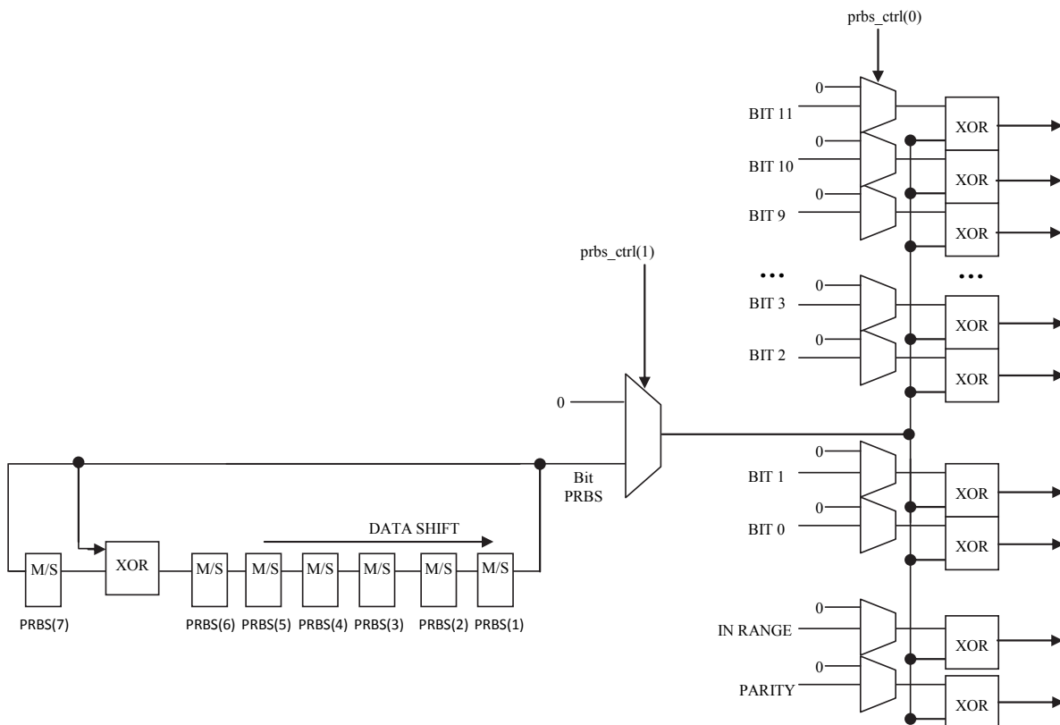
Figure 22. PRBS encoding data
