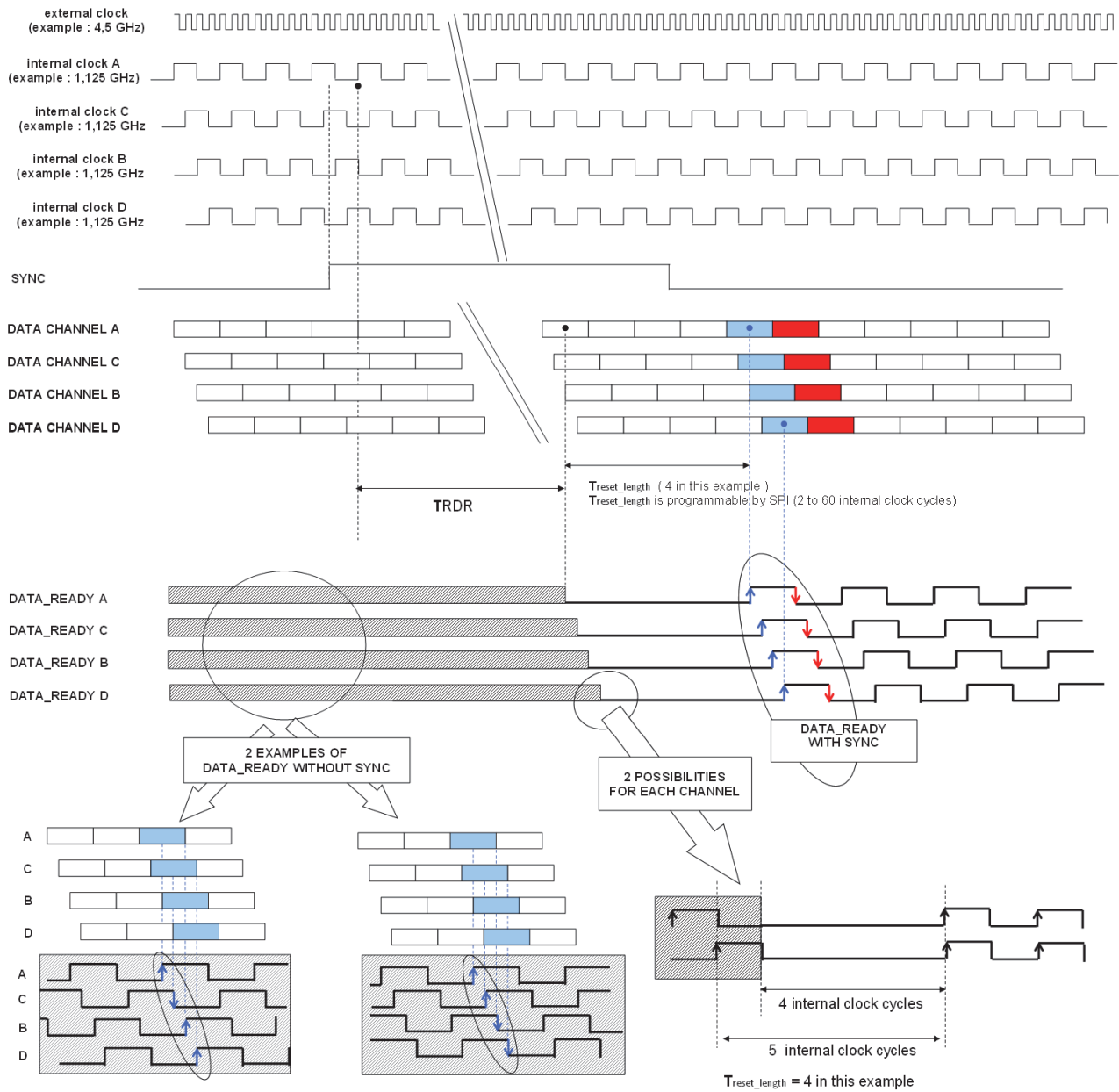
Figure 21. SYNC Timing
