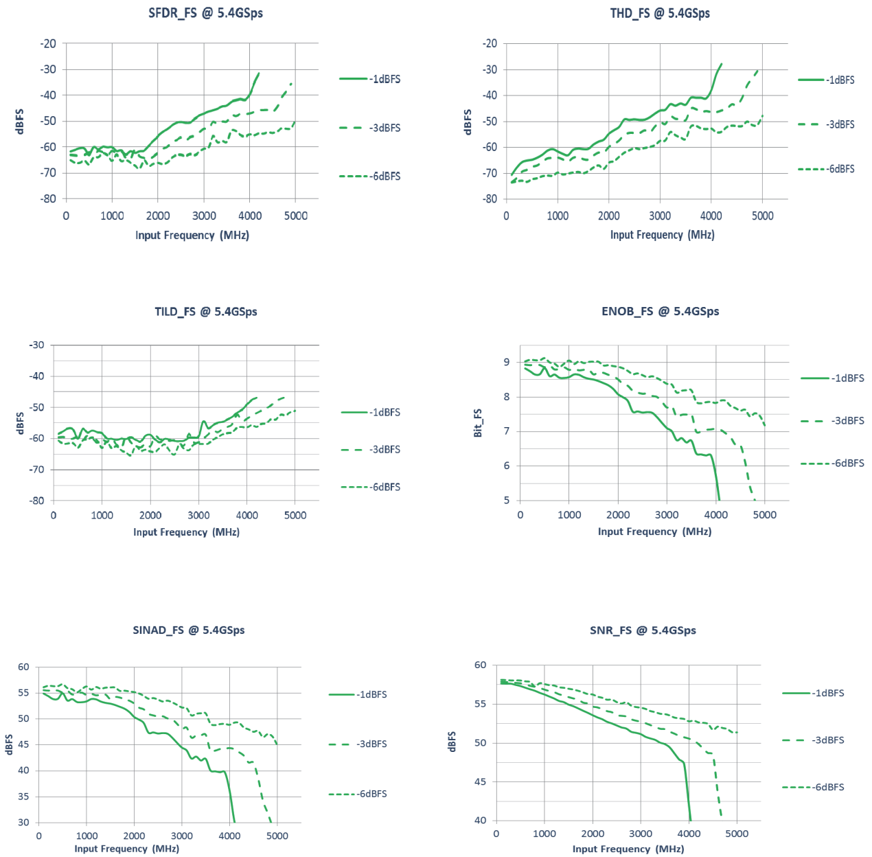
Figure 31. : SFDR, THD, ENOB, SINAD and SNR performances at versus input frequency at 5.4GSps
