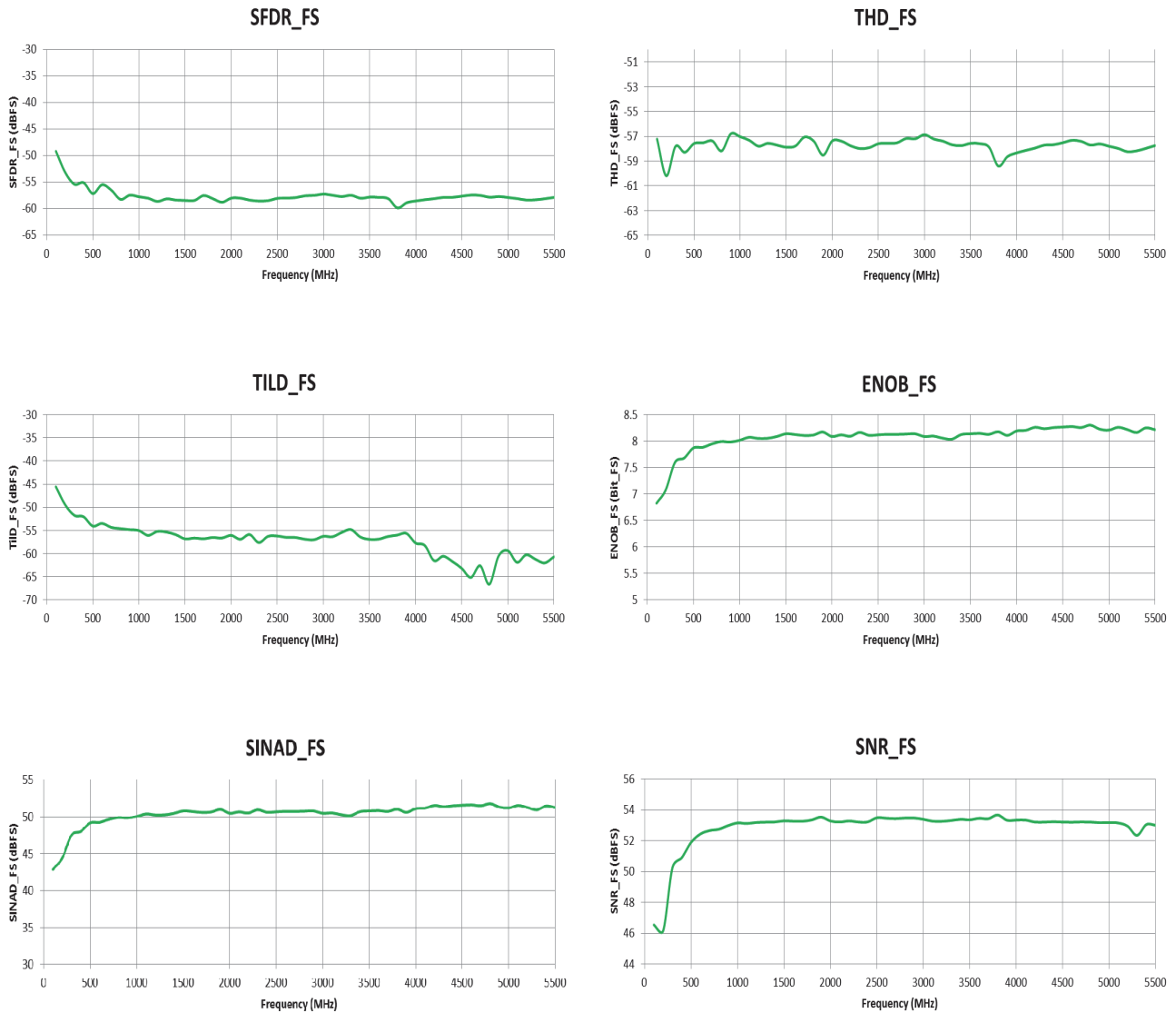
Typical supplies - at ambient temperature - 4 cores interleaved (Staggered mode).
