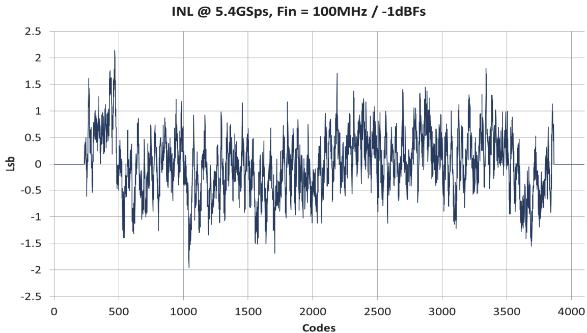
Figure 29. INL performances at 5.4GSps
