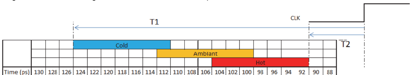
Figure 9. SYNC edges forbidden zone versus temperature
