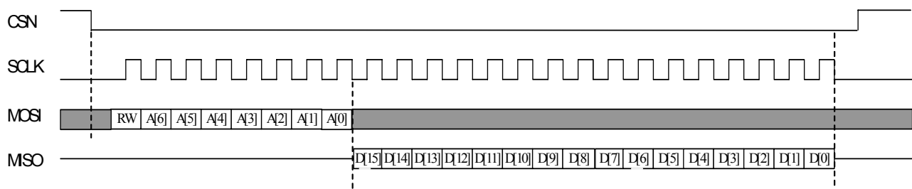
Figure 16. SPI reading
