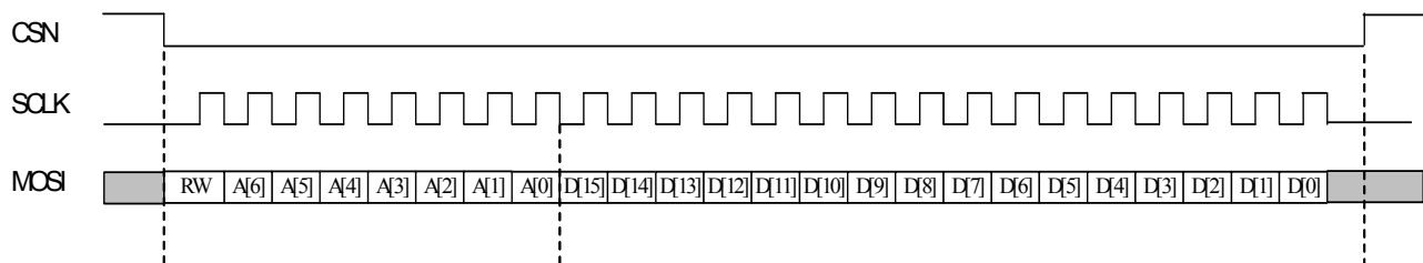
Figure 15. SPI writing (16-bit register)
