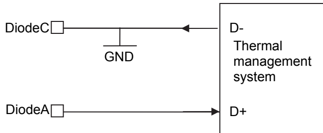
Figure 27. Junction temperature monitoring diode system
