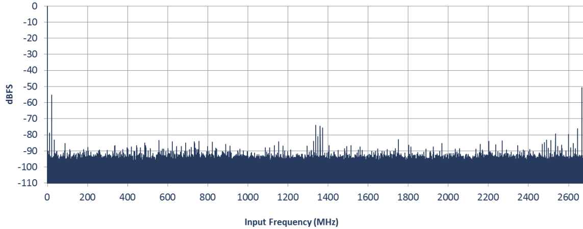
Figure 38. FFT at 5.4GSps and F_{in} = 2690\text{MHz} / -1\text{dBFS}
