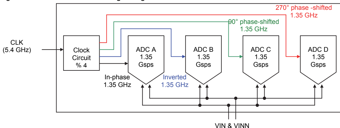
Figure 3. Internal interleaving configuration
