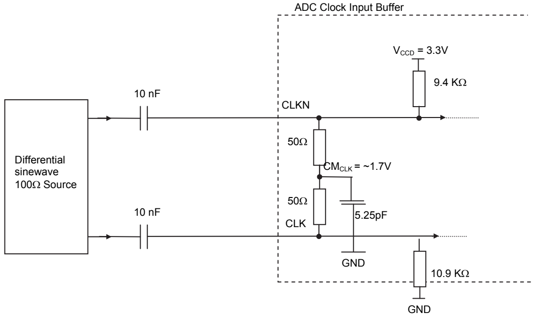
Figure 56. Differential clock input implementation (AC coupled)
