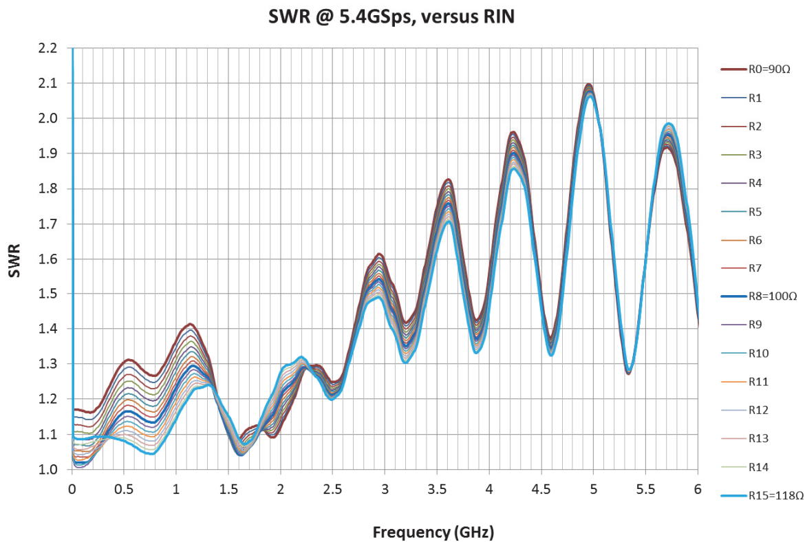
Figure 48. VSWR measurement on board with socket
