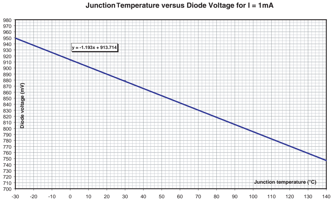
Figure 5-6. ADC DIODE Characteristics
