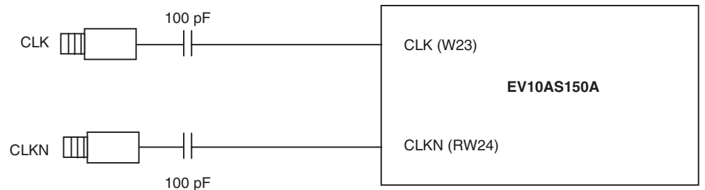
Figure 2-3. Differential Clock Inputs Implementation
