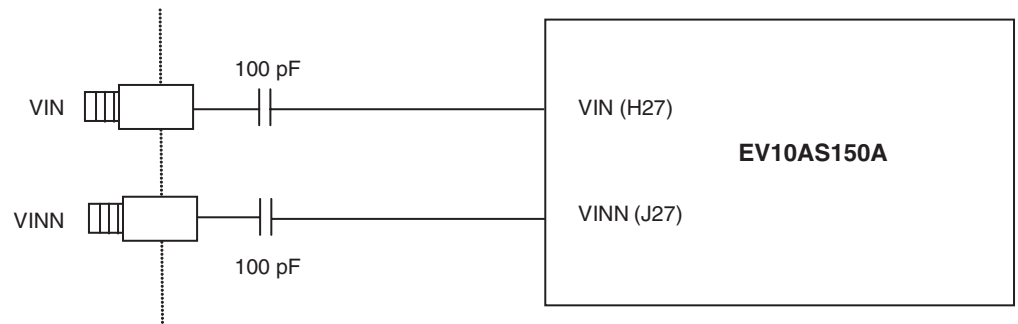
Figure 2-2. Differential Analog Inputs Implementation
