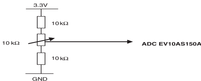
Figure 5-3. CLKDACTRL Potentiometer
