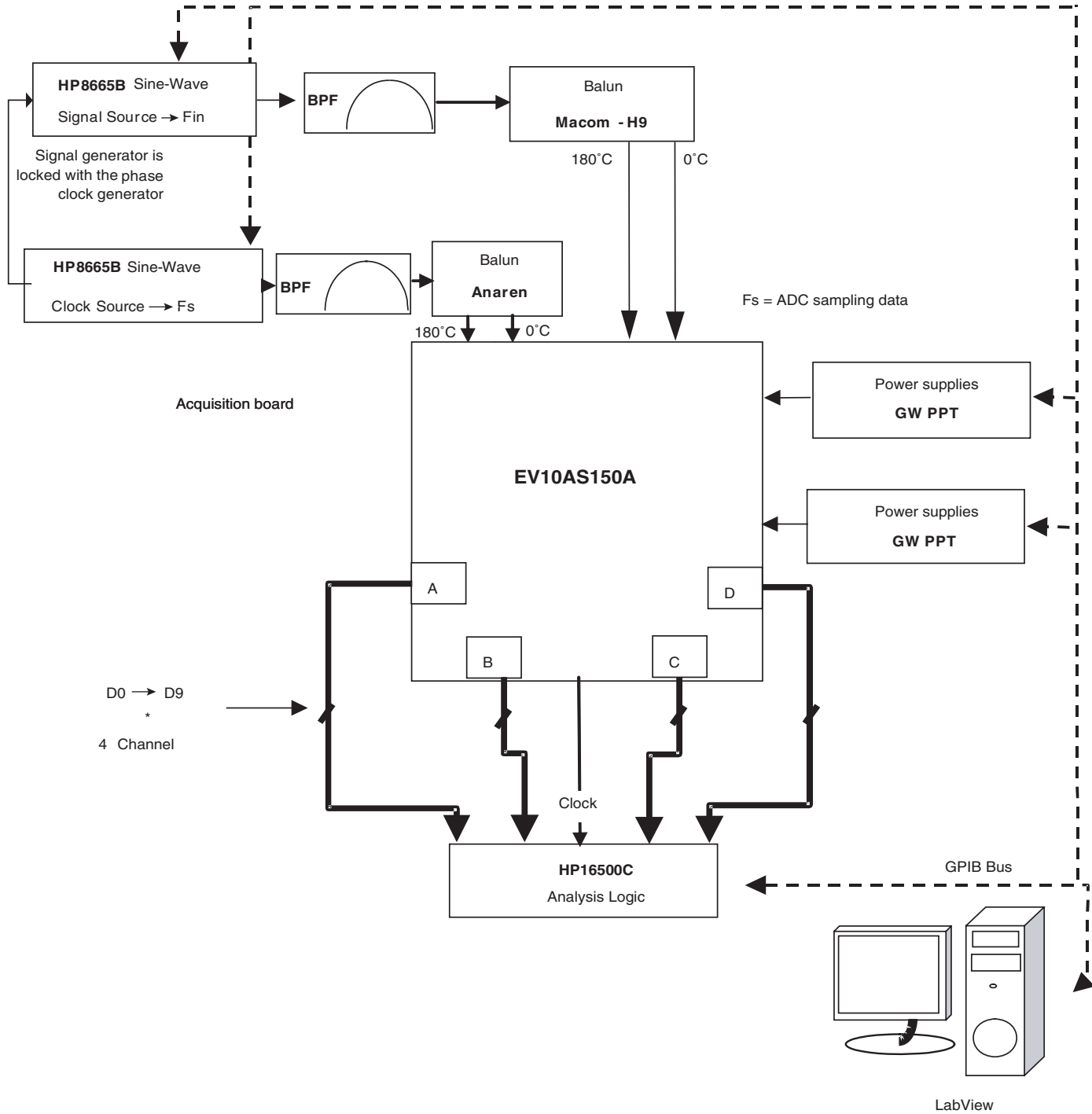
Figure 5-7. Test Bench Description
