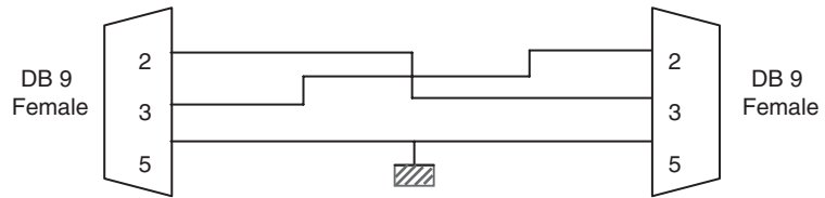
Figure 4-10. Crossed RS232 Cable
