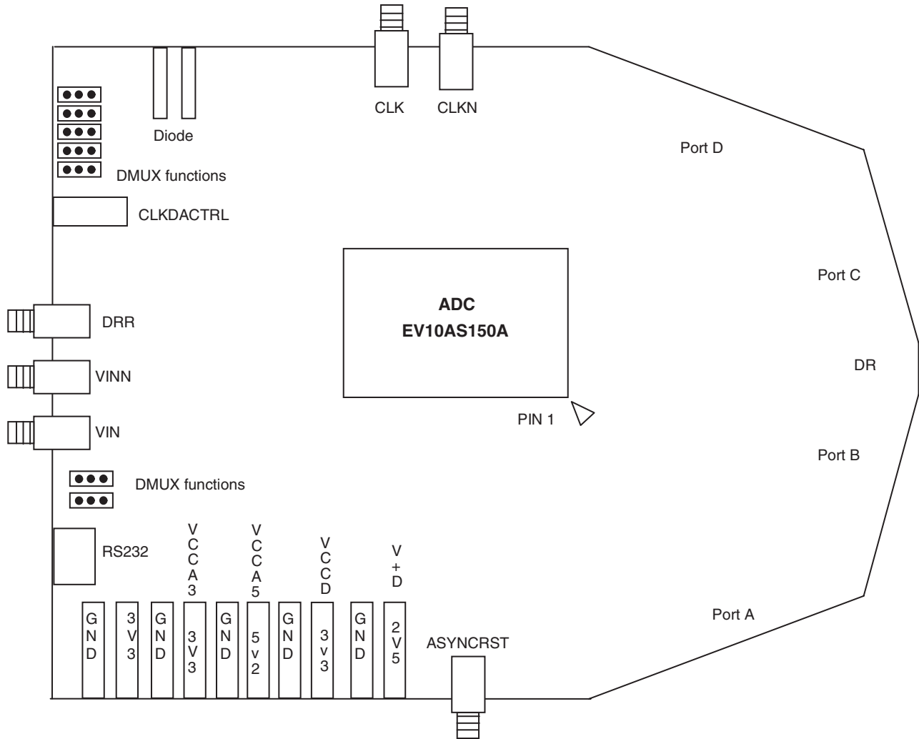
Figure 1-1. ADC EV10AS150A-EB Evaluation Board Simplified Schematic
